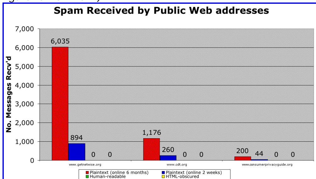
Figure 2 - Messages received by addresses on the public Web (select figure for full view.)
