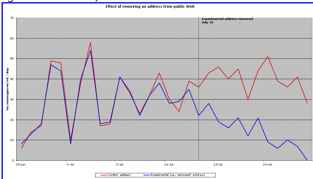
Figure 4 - Effect of removing an address from the public Web (select figure for full view.)
